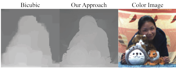
Fig. 6 Comparison between our method and bicubic upsampling on real scenes. The disparity map is upsampled from 320 \times 240 to 640 \times 480 . Our method preserves sharp edges and maintains smoothness, which is critical to reliable DoF synthesis.
